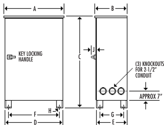
PADMOUNT
